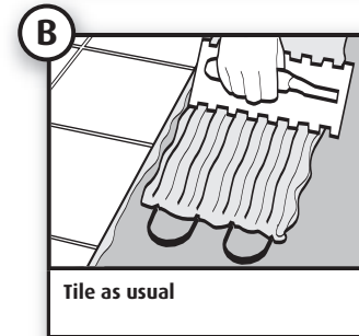
Use correct adhesive and grout
